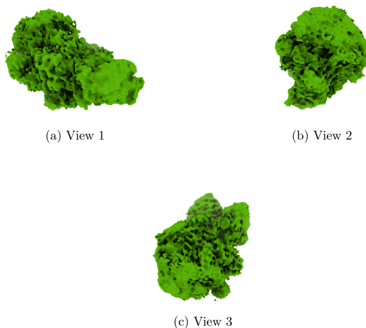
Figure 4: Isosurface at threshold=0.050400. Views generated by ChimeraX at a the following X, Y, Z angles: View 1 (0, -90, -90), View 2 (-90, 0, -90), View 3 (0, 0, 0).
