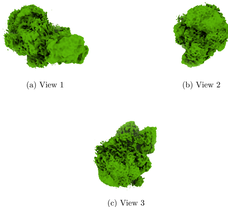
Figure 4: Isosurface at threshold=0.039900. Views generated by ChimeraX at a the following X, Y, Z angles: View 1 (0, -90, -90), View 2 (-90, 0, -90), View 3 (0, 0, 0).
