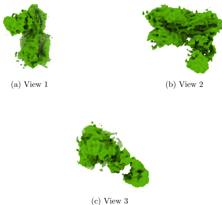
Figure 4: Isosurface at threshold=0.004600. Views generated by ChimeraX at a the following X, Y, Z angles: View 1 (0, -90, -90), View 2 (-90, 0, -90), View 3 (0, 0, 0).
