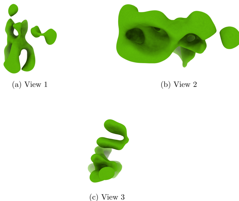
Figure 4: Isosurface at threshold=0.023700. Views generated by ChimeraX at a the following X, Y, Z angles: View 1 (0, -90, -90), View 2 (-90, 0, -90), View 3 (0, 0, 0).
