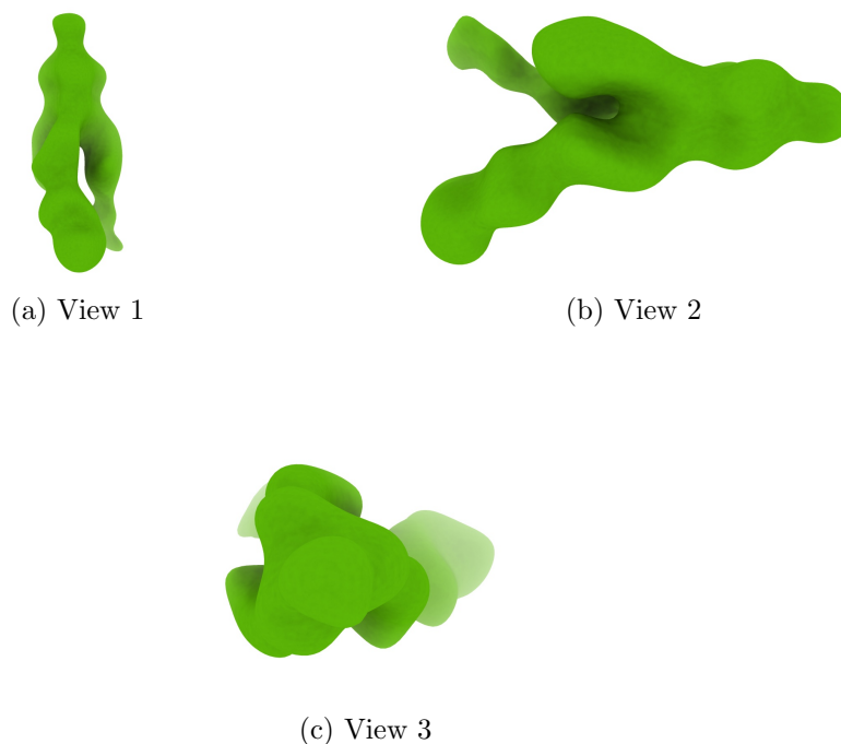
Figure 4: Isosurface at threshold=0.024200. Views generated by ChimeraX at a the following X, Y, Z angles: View 1 (0, -90, -90), View 2 (-90, 0, -90), View 3 (0, 0, 0).
