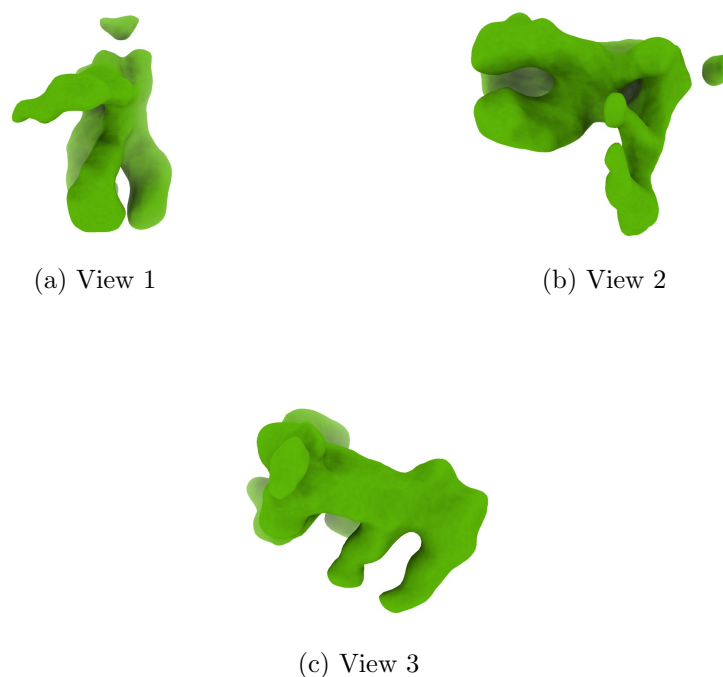
Figure 4: Isosurface at threshold=0.020600. Views generated by ChimeraX at a the following X, Y, Z angles: View 1 (0, -90, -90), View 2 (-90, 0, -90), View 3 (0, 0, 0).
