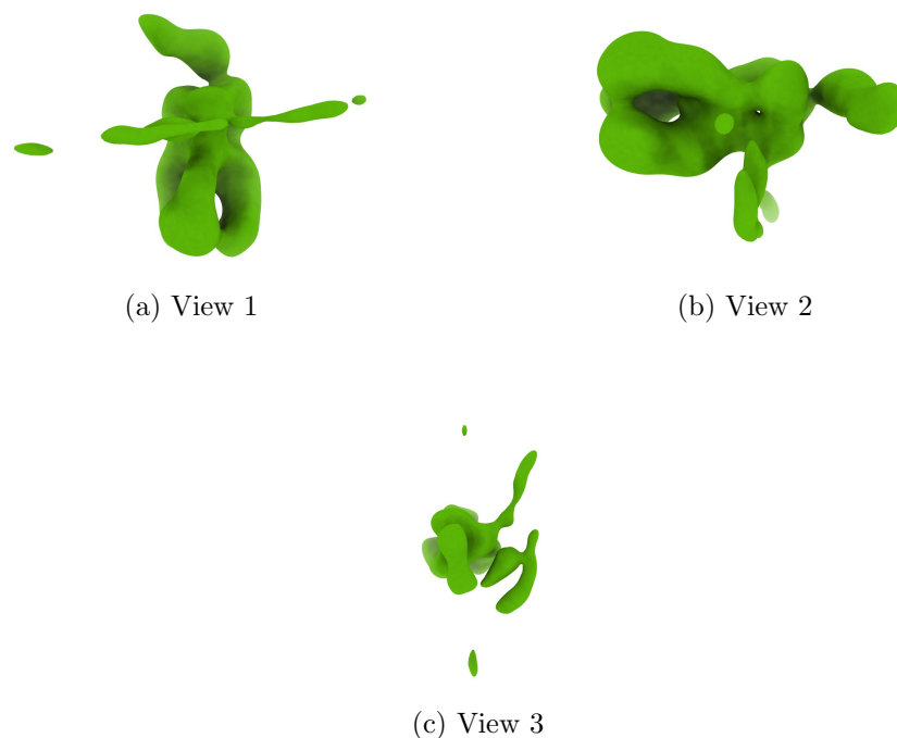
Figure 4: Isosurface at threshold=0.015800. Views generated by ChimeraX at a the following X, Y, Z angles: View 1 (0, -90, -90), View 2 (-90, 0, -90), View 3 (0, 0, 0).
