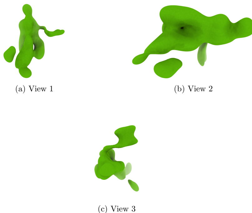
Figure 4: Isosurface at threshold=0.025100. Views generated by ChimeraX at a the following X, Y, Z angles: View 1 (0, -90, -90), View 2 (-90, 0, -90), View 3 (0, 0, 0).
