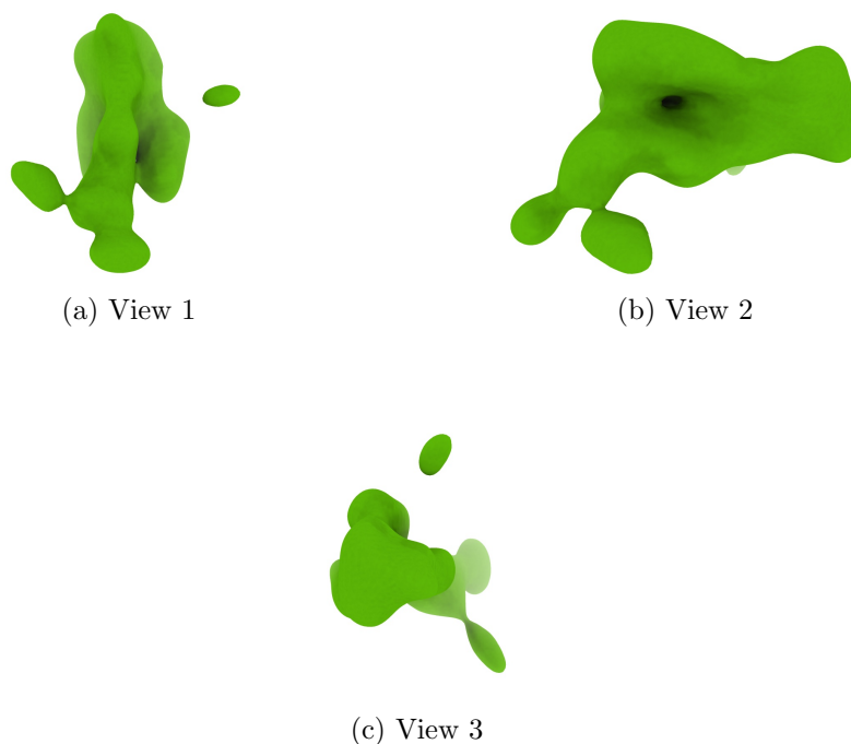
Figure 4: Isosurface at threshold=0.019800. Views generated by ChimeraX at a the following X, Y, Z angles: View 1 (0, -90, -90), View 2 (-90, 0, -90), View 3 (0, 0, 0).
