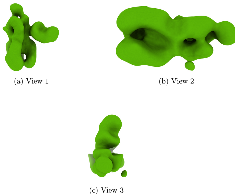
Figure 4: Isosurface at threshold=0.011700. Views generated by ChimeraX at a the following X, Y, Z angles: View 1 (0, -90, -90), View 2 (-90, 0, -90), View 3 (0, 0, 0).
