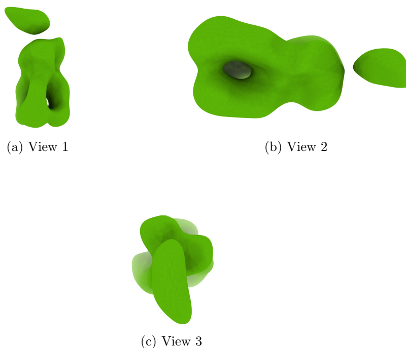
Figure 4: Isosurface at threshold=0.016800. Views generated by ChimeraX at a the following X, Y, Z angles: View 1 (0, -90, -90), View 2 (-90, 0, -90), View 3 (0, 0, 0).
