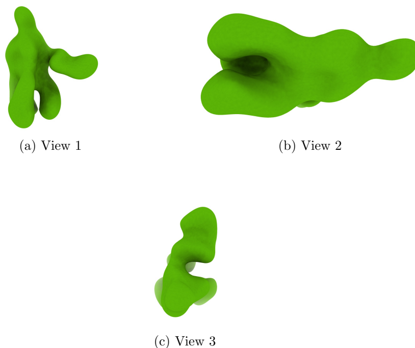
Figure 4: Isosurface at threshold=0.022900. Views generated by ChimeraX at a the following X, Y, Z angles: View 1 (0, -90, -90), View 2 (-90, 0, -90), View 3 (0, 0, 0).
