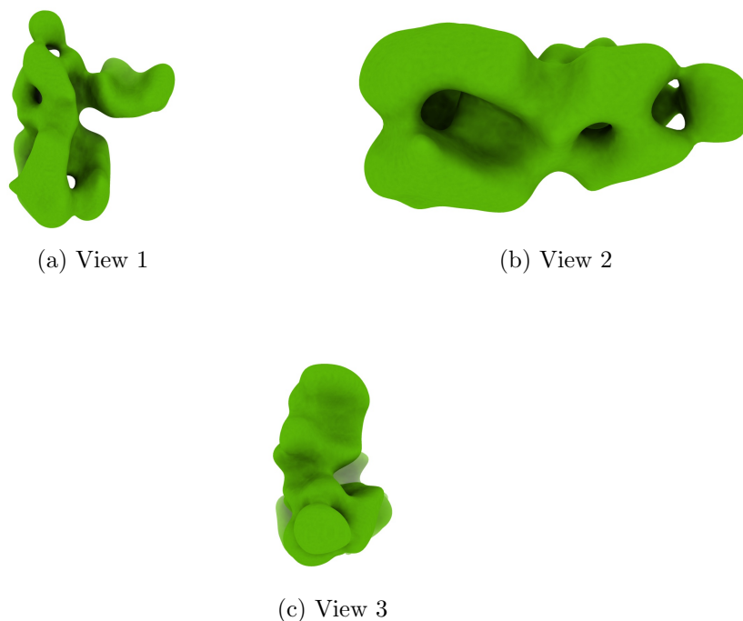
Figure 4: Isosurface at threshold=0.013300. Views generated by ChimeraX at a the following X, Y, Z angles: View 1 (0, -90, -90), View 2 (-90, 0, -90), View 3 (0, 0, 0).
