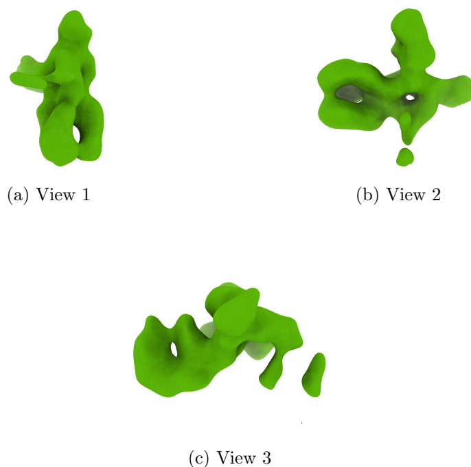
Figure 4: Isosurface at threshold=0.017900. Views generated by ChimeraX at a the following X, Y, Z angles: View 1 (0, -90, -90), View 2 (-90, 0, -90), View 3 (0, 0, 0).
