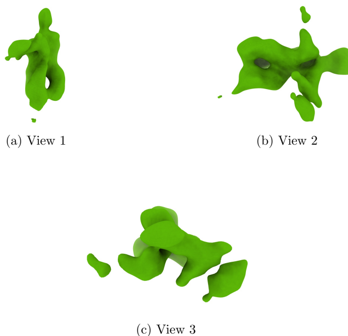
Figure 4: Isosurface at threshold=0.022900. Views generated by ChimeraX at a the following X, Y, Z angles: View 1 (0, -90, -90), View 2 (-90, 0, -90), View 3 (0, 0, 0).
