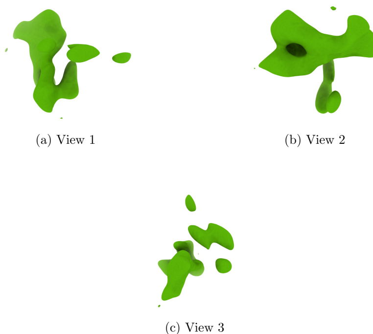
Figure 4: Isosurface at threshold=0.025200. Views generated by ChimeraX at a the following X, Y, Z angles: View 1 (0, -90, -90), View 2 (-90, 0, -90), View 3 (0, 0, 0).
