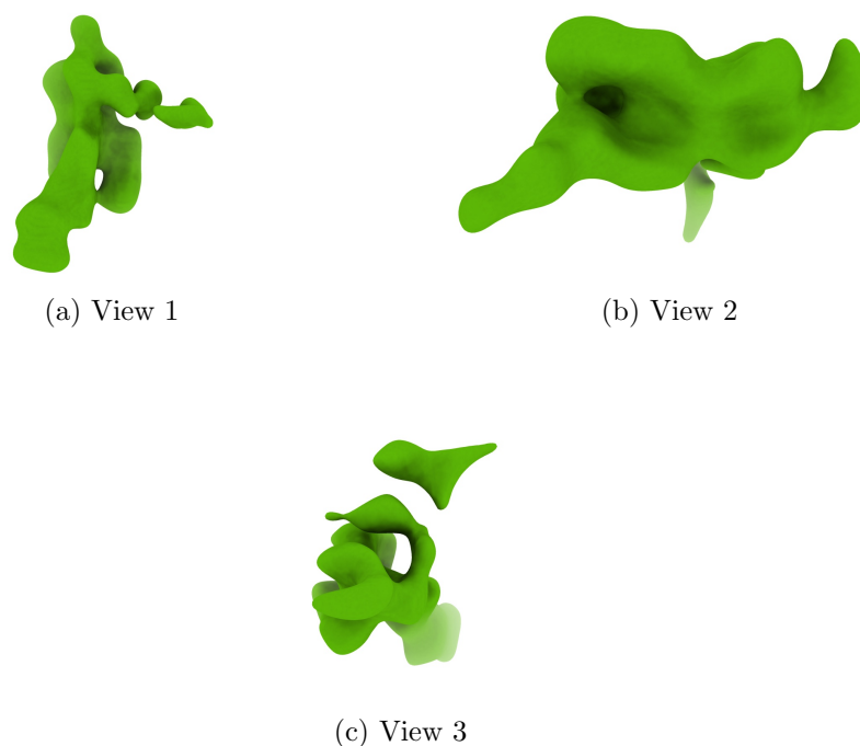
Figure 4: Isosurface at threshold=0.013900. Views generated by ChimeraX at a the following X, Y, Z angles: View 1 (0, -90, -90), View 2 (-90, 0, -90), View 3 (0, 0, 0).
