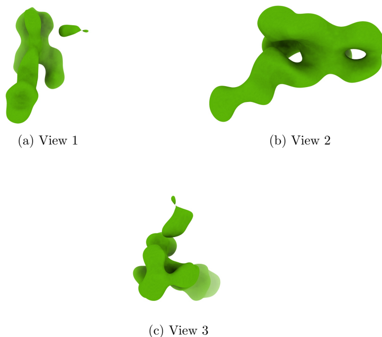
Figure 4: Isosurface at threshold=0.023200. Views generated by ChimeraX at a the following X, Y, Z angles: View 1 (0, -90, -90), View 2 (-90, 0, -90), View 3 (0, 0, 0).
