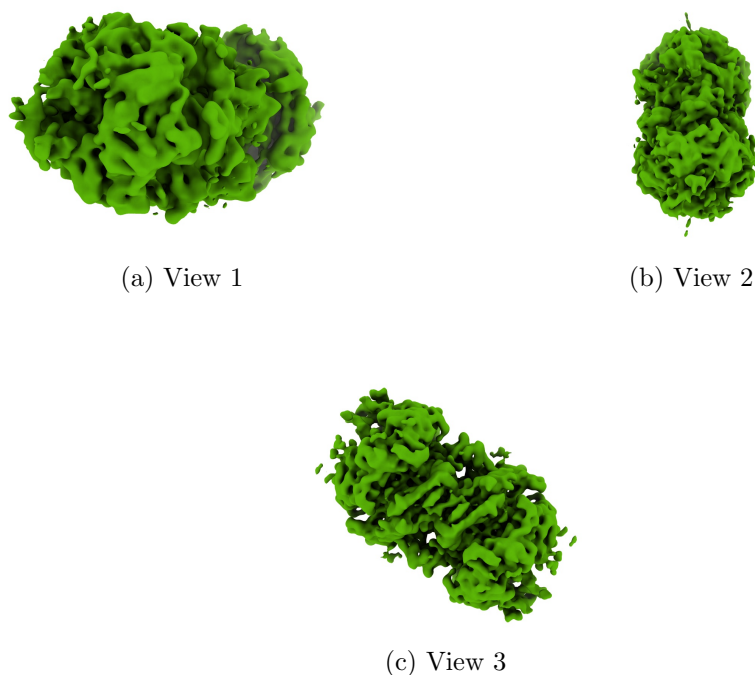
Figure 4: Isosurface at threshold=0.645000. Views generated by ChimeraX at a the following X, Y, Z angles: View 1 (0, -90, -90), View 2 (-90, 0, -90), View 3 (0, 0, 0).
