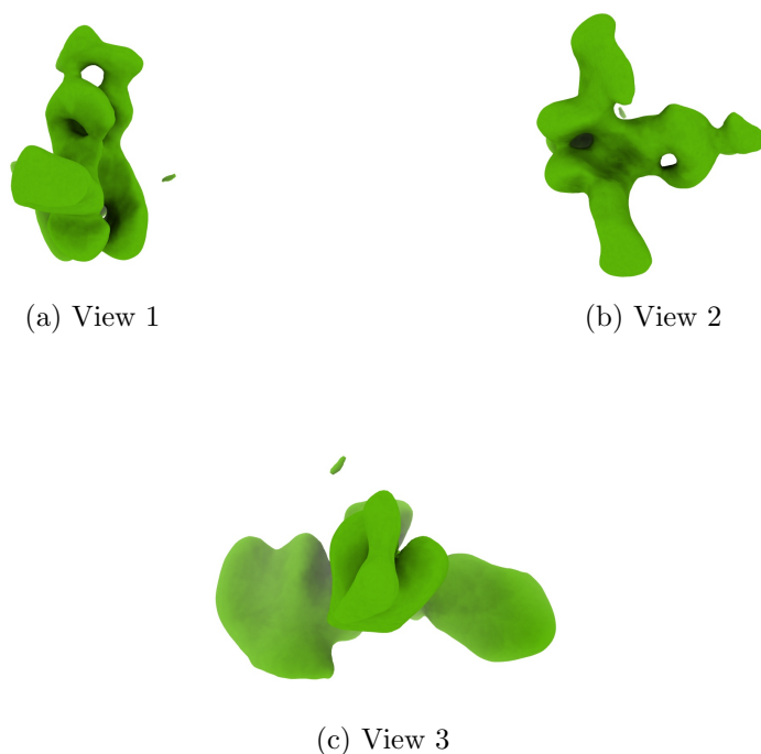
Figure 4: Isosurface at threshold=0.023400. Views generated by ChimeraX at a the following X, Y, Z angles: View 1 (0, -90, -90), View 2 (-90, 0, -90), View 3 (0, 0, 0).
