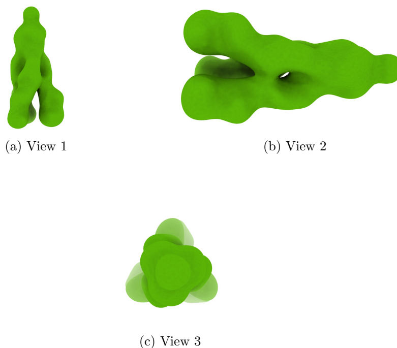
Figure 4: Isosurface at threshold=0.019500. Views generated by ChimeraX at a the following X, Y, Z angles: View 1 (0, -90, -90), View 2 (-90, 0, -90), View 3 (0, 0, 0).
