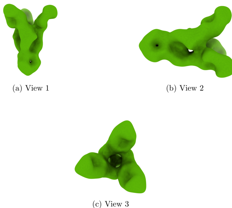
Figure 4: Isosurface at threshold=0.013300. Views generated by ChimeraX at a the following X, Y, Z angles: View 1 (0, -90, -90), View 2 (-90, 0, -90), View 3 (0, 0, 0).
