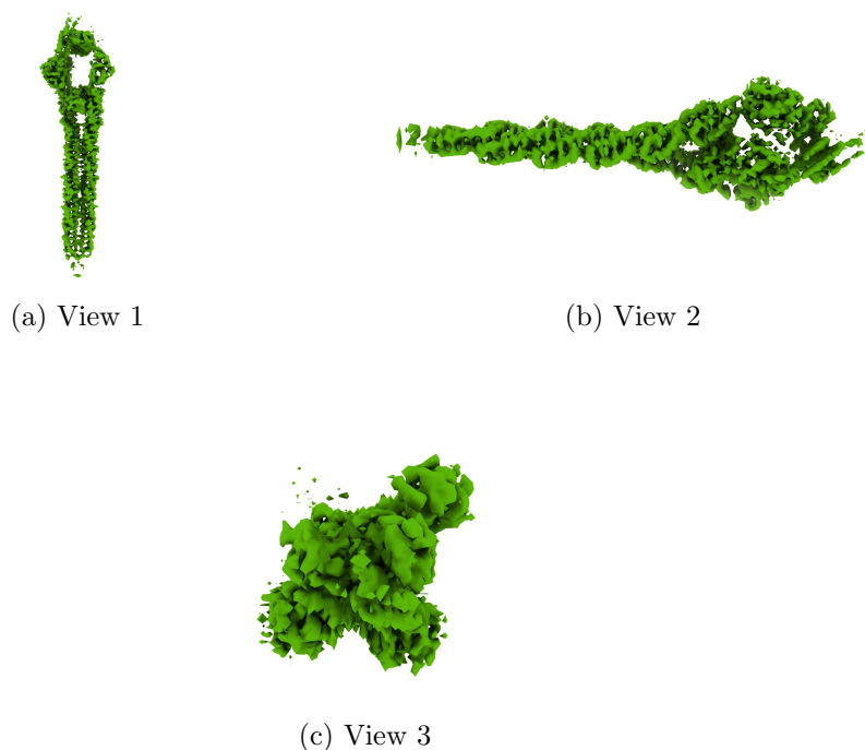
Figure 4: Isosurface at threshold=0.330000. Views generated by ChimeraX at a the following X, Y, Z angles: View 1 (0, -90, -90), View 2 (-90, 0, -90), View 3 (0, 0, 0).
