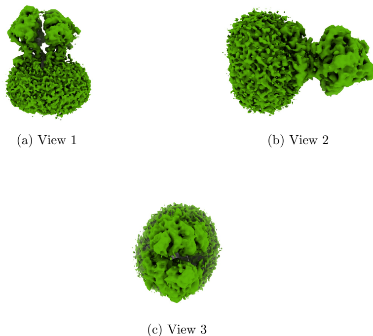
Figure 4: Isosurface at threshold=0.061100. Views generated by ChimeraX at a the following X, Y, Z angles: View 1 (0, -90, -90), View 2 (-90, 0, -90), View 3 (0, 0, 0).
