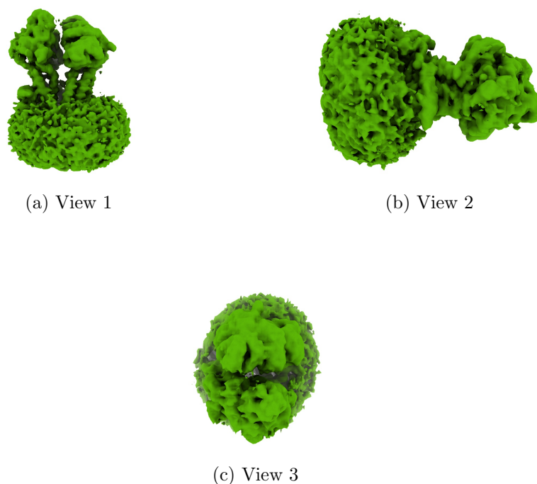
Figure 4: Isosurface at threshold=0.058400. Views generated by ChimeraX at a the following X, Y, Z angles: View 1 (0, -90, -90), View 2 (-90, 0, -90), View 3 (0, 0, 0).
