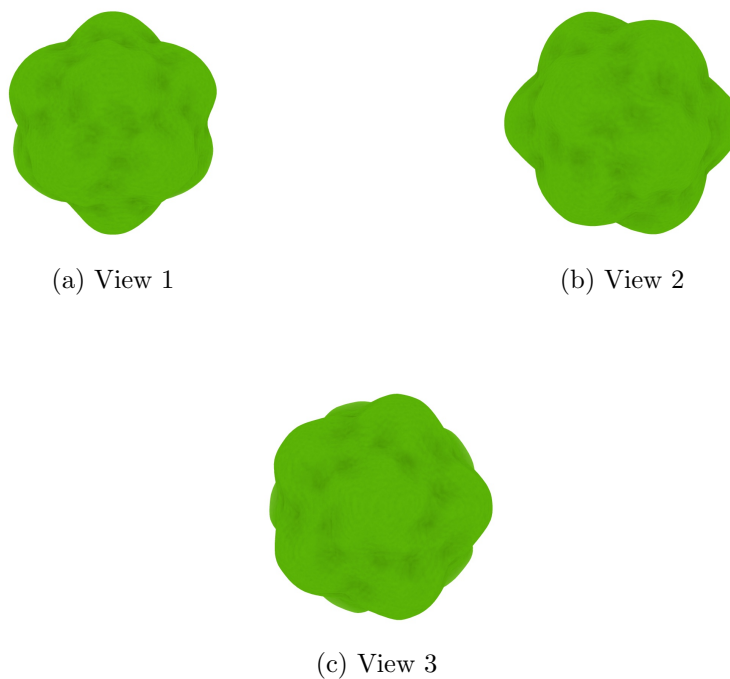
Figure 4: Isosurface at threshold=4.790000. Views generated by ChimeraX at a the following X, Y, Z angles: View 1 (0, -90, -90), View 2 (-90, 0, -90), View 3 (0, 0, 0).
