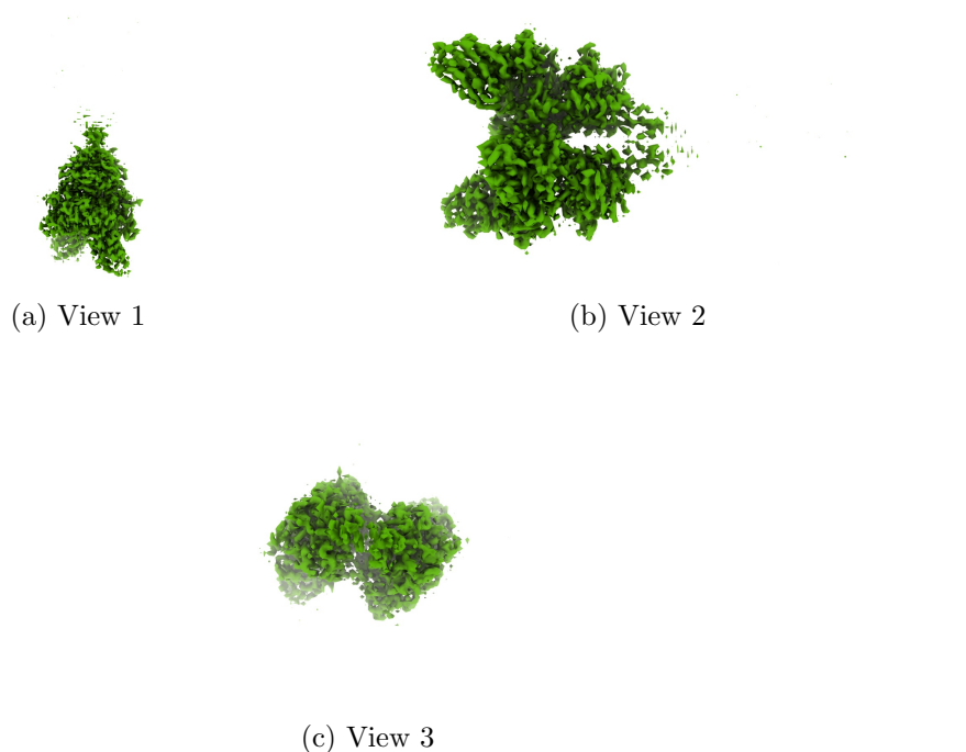
Figure 4: Isosurface at threshold=0.338000. Views generated by ChimeraX at a the following X, Y, Z angles: View 1 (0, -90, -90), View 2 (-90, 0, -90), View 3 (0, 0, 0).
