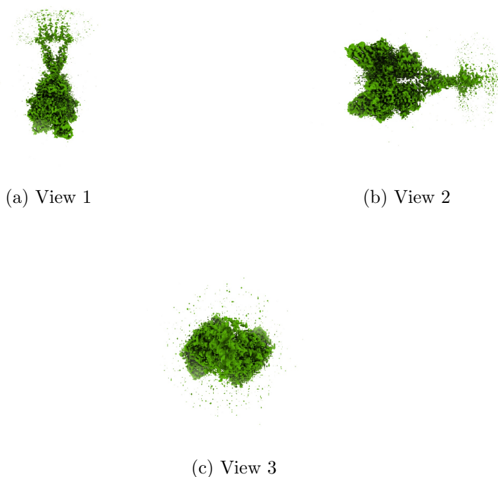
Figure 4: Isosurface at threshold=0.242000. Views generated by ChimeraX at a the following X, Y, Z angles: View 1 (0, -90, -90), View 2 (-90, 0, -90), View 3 (0, 0, 0).
