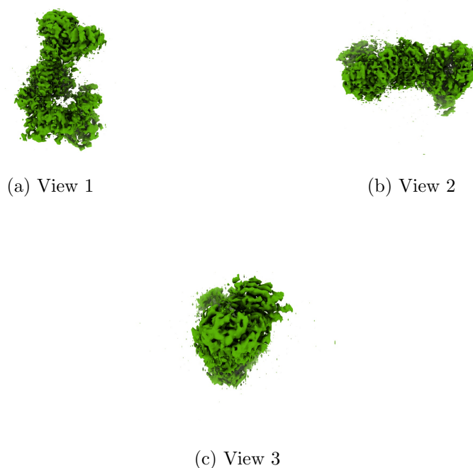
Figure 4: Isosurface at threshold=0.135000. Views generated by ChimeraX at a the following X, Y, Z angles: View 1 (0, -90, -90), View 2 (-90, 0, -90), View 3 (0, 0, 0).
