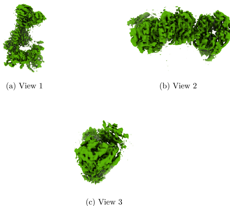
Figure 4: Isosurface at threshold=0.141000. Views generated by ChimeraX at a the following X, Y, Z angles: View 1 (0, -90, -90), View 2 (-90, 0, -90), View 3 (0, 0, 0).
