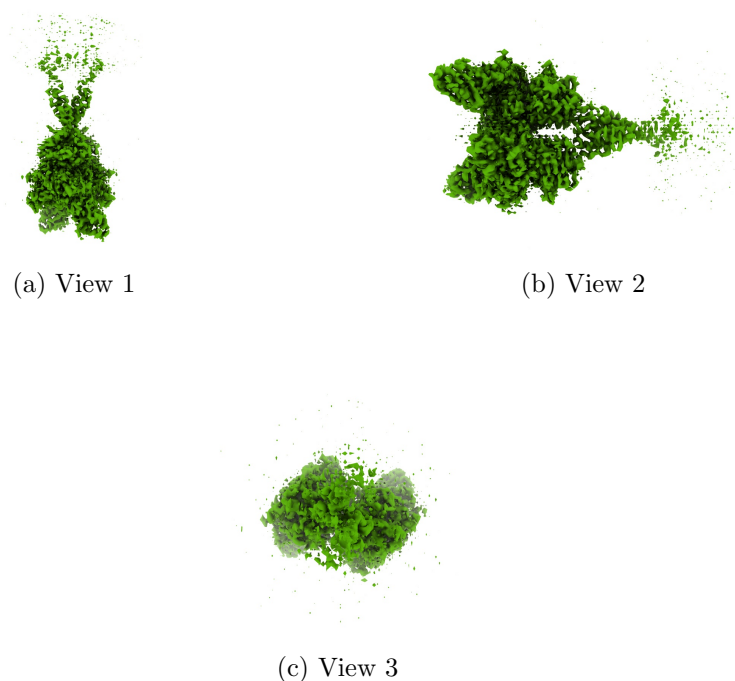
Figure 4: Isosurface at threshold=0.264000. Views generated by ChimeraX at a the following X, Y, Z angles: View 1 (0, -90, -90), View 2 (-90, 0, -90), View 3 (0, 0, 0).
