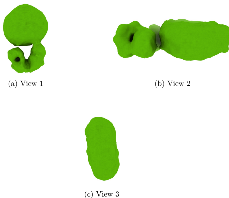
Figure 4: Isosurface at threshold=0.088600. Views generated by ChimeraX at a the following X, Y, Z angles: View 1 (0, -90, -90), View 2 (-90, 0, -90), View 3 (0, 0, 0).
