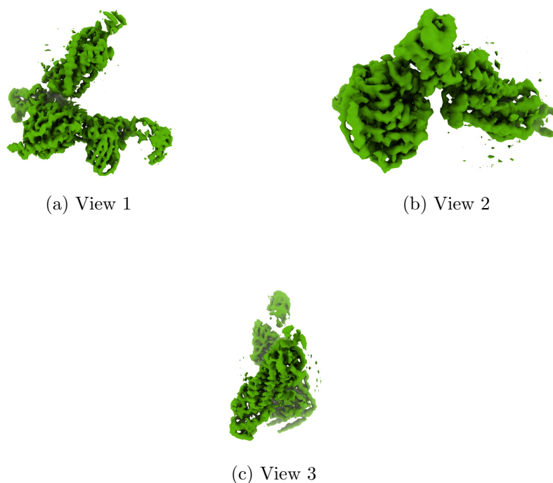
Figure 4: Isosurface at threshold=0.106000. Views generated by ChimeraX at a the following X, Y, Z angles: View 1 (0, -90, -90), View 2 (-90, 0, -90), View 3 (0, 0, 0).
