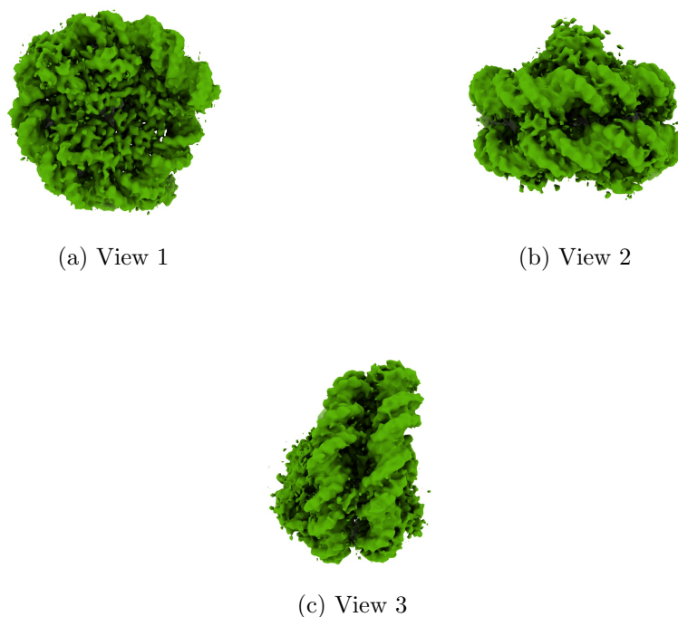
Figure 4: Isosurface at threshold=0.060000. Views generated by ChimeraX at the following X, Y, Z angles: View 1 (0, -90, -90), View 2 (-90, 0, -90), View 3 (0, 0, 0).
