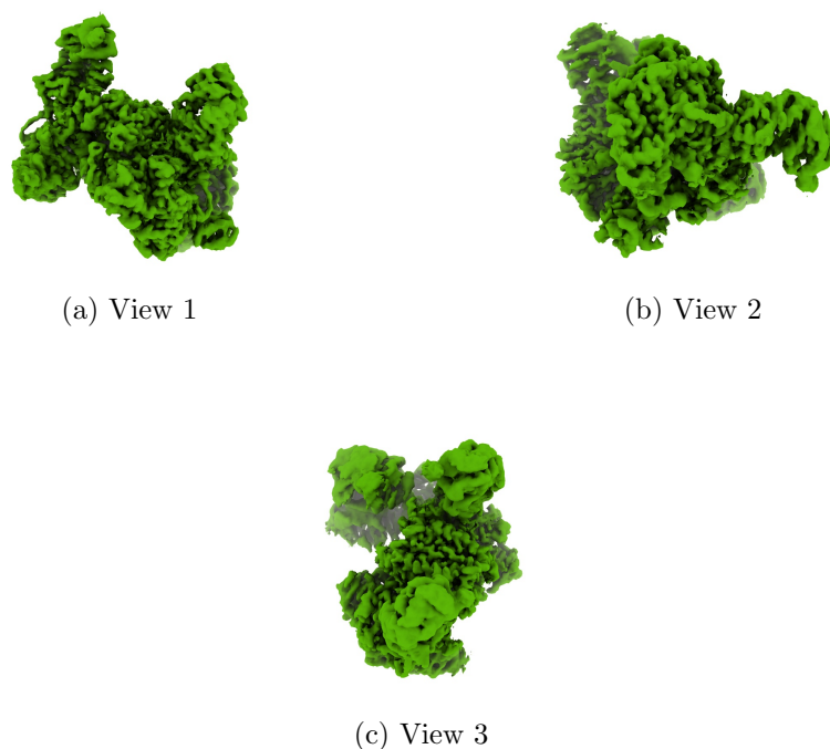
Figure 4: Isosurface at threshold=0.065800. Views generated by ChimeraX at a the following X, Y, Z angles: View 1 (0, -90, -90), View 2 (-90, 0, -90), View 3 (0, 0, 0).
