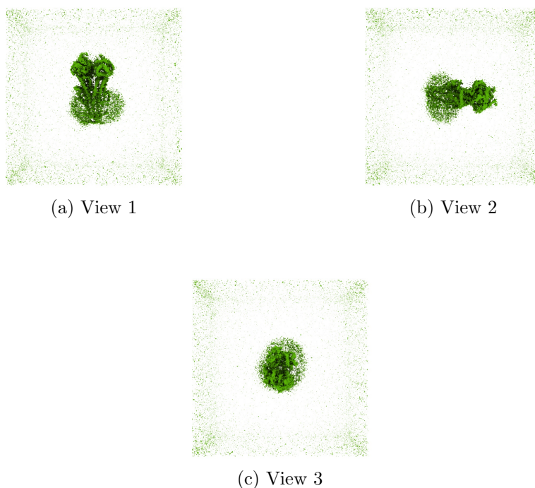
Figure 4: Isosurface at threshold=0.117000. Views generated by ChimeraX at a the following X, Y, Z angles: View 1 (0, -90, -90), View 2 (-90, 0, -90), View 3 (0, 0, 0).
