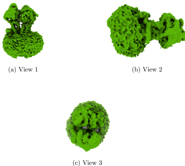
Figure 4: Isosurface at threshold=0.070400. Views generated by ChimeraX at a the following X, Y, Z angles: View 1 (0, -90, -90), View 2 (-90, 0, -90), View 3 (0, 0, 0).
