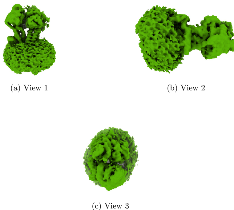
Figure 4: Isosurface at threshold=0.070300. Views generated by ChimeraX at a the following X, Y, Z angles: View 1 (0, -90, -90), View 2 (-90, 0, -90), View 3 (0, 0, 0).
