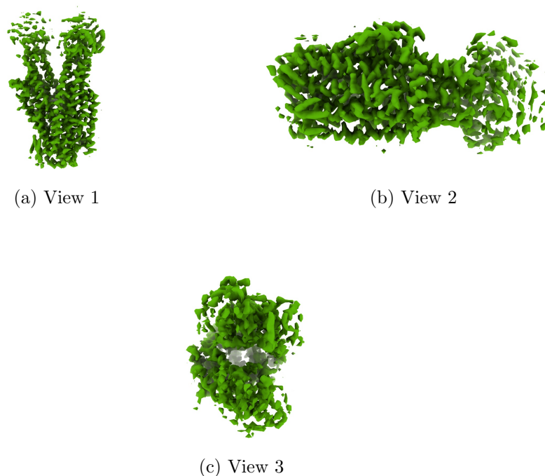
Figure 4: Isosurface at threshold=0.195000. Views generated by ChimeraX at a the following X, Y, Z angles: View 1 (0, -90, -90), View 2 (-90, 0, -90), View 3 (0, 0, 0).
