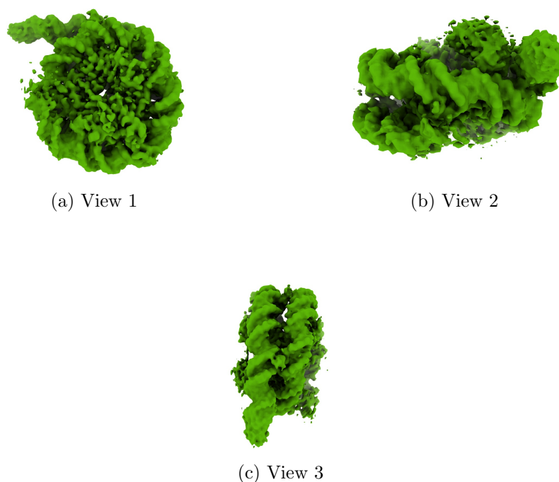
Figure 4: Isosurface at threshold=0.071100. Views generated by ChimeraX at a the following X, Y, Z angles: View 1 (0, -90, -90), View 2 (-90, 0, -90), View 3 (0, 0, 0).
