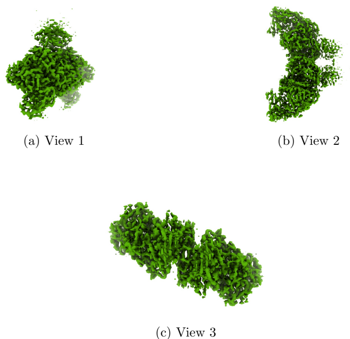
Figure 4: Isosurface at threshold=0.860000. Views generated by ChimeraX at a the following X, Y, Z angles: View 1 (0, -90, -90), View 2 (-90, 0, -90), View 3 (0, 0, 0).
