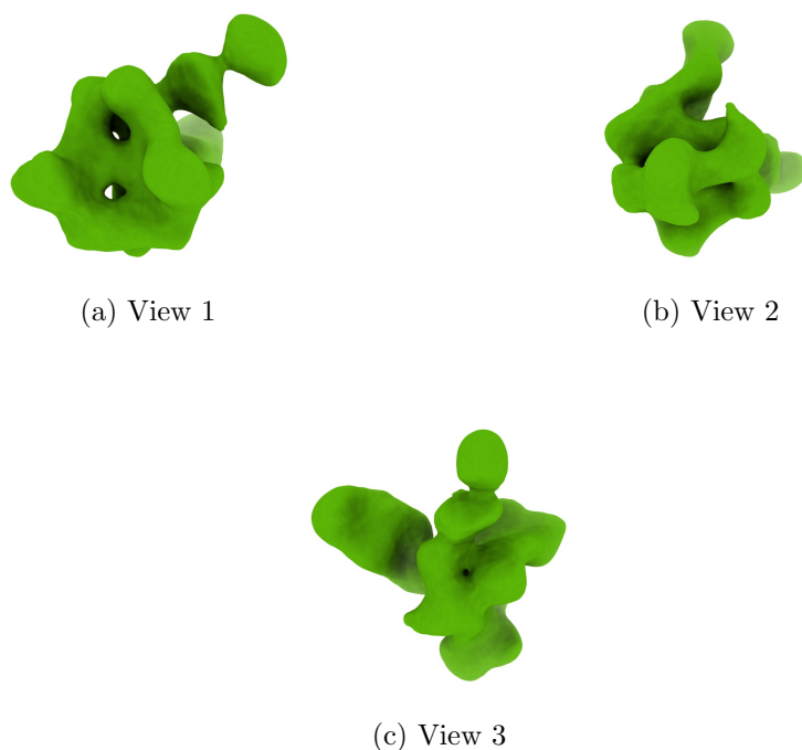
Figure 4: Isosurface at threshold=0.016200. Views generated by ChimeraX at a the following X, Y, Z angles: View 1 (0, -90, -90), View 2 (-90, 0, -90), View 3 (0, 0, 0).
