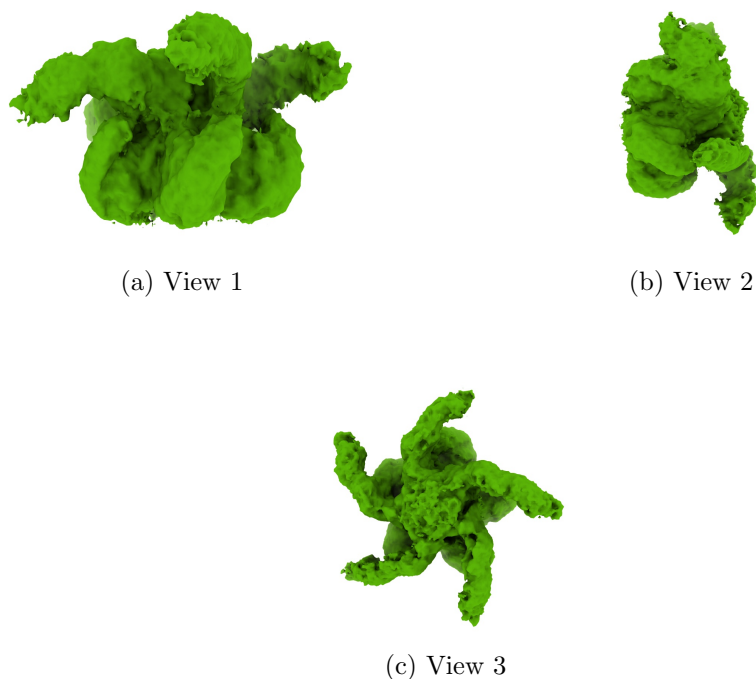
Figure 4: Isosurface at threshold=0.004750. Views generated by ChimeraX at a the following X, Y, Z angles: View 1 (0, -90, -90), View 2 (-90, 0, -90), View 3 (0, 0, 0).
