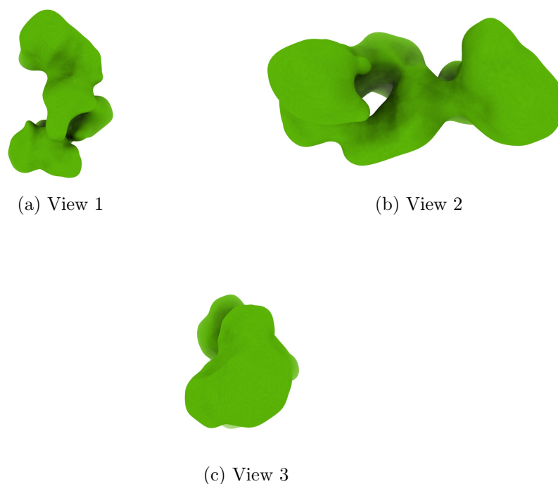
Figure 4: Isosurface at threshold=2.350000. Views generated by ChimeraX at a the following X, Y, Z angles: View 1 (0, -90, -90), View 2 (-90, 0, -90), View 3 (0, 0, 0).
