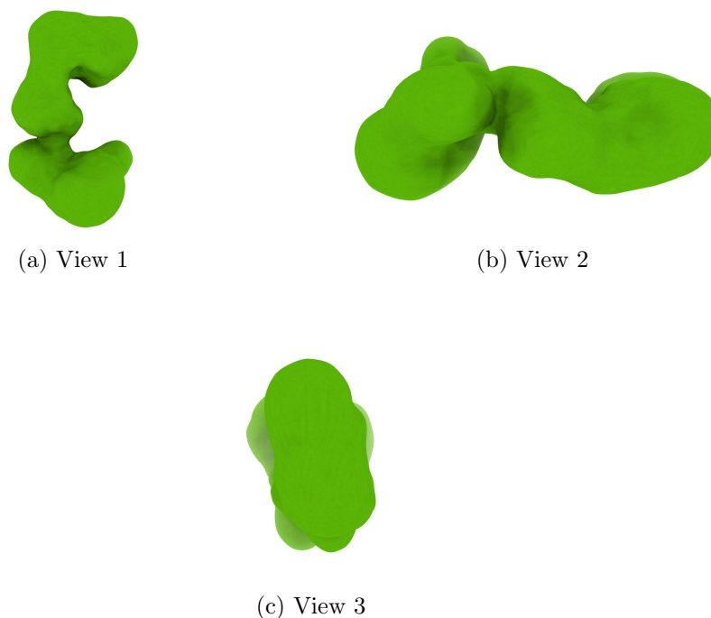
Figure 4: Isosurface at threshold=1.810000. Views generated by ChimeraX at a the following X, Y, Z angles: View 1 (0, -90, -90), View 2 (-90, 0, -90), View 3 (0, 0, 0).
