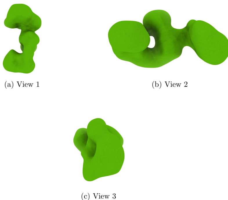
Figure 4: Isosurface at threshold=2.590000. Views generated by ChimeraX at a the following X, Y, Z angles: View 1 (0, -90, -90), View 2 (-90, 0, -90), View 3 (0, 0, 0).
