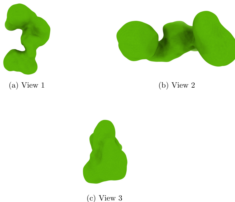
Figure 4: Isosurface at threshold=2.830000. Views generated by ChimeraX at a the following X, Y, Z angles: View 1 (0, -90, -90), View 2 (-90, 0, -90), View 3 (0, 0, 0).
