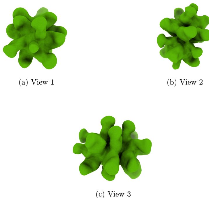
Figure 4: Isosurface at threshold=0.039000. Views generated by ChimeraX at a the following X, Y, Z angles: View 1 (0, -90, -90), View 2 (-90, 0, -90), View 3 (0, 0, 0).
