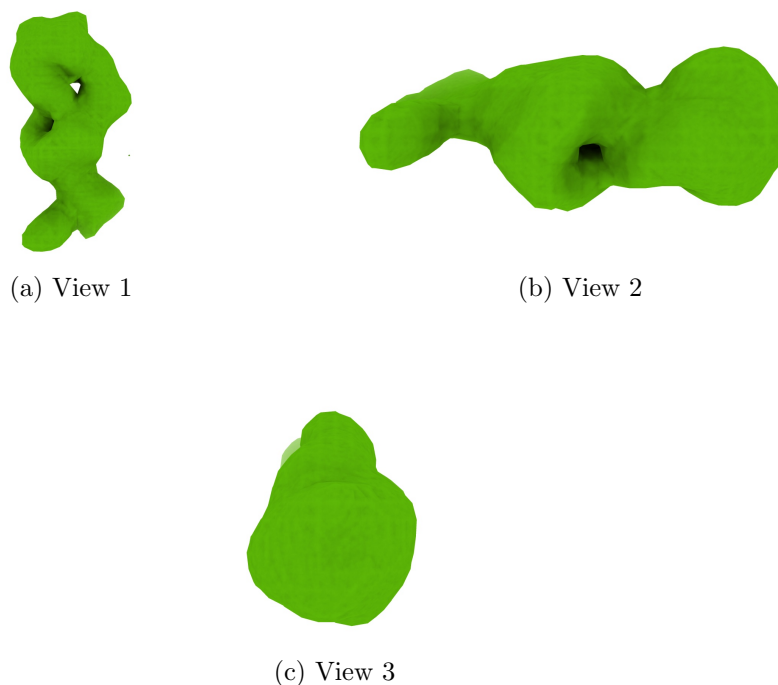
Figure 4: Isosurface at threshold=0.533000. Views generated by ChimeraX at a the following X, Y, Z angles: View 1 (0, -90, -90), View 2 (-90, 0, -90), View 3 (0, 0, 0).
