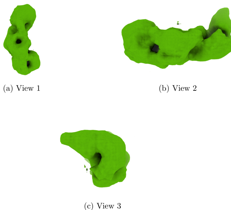
Figure 4: Isosurface at threshold=0.168000. Views generated by ChimeraX at a the following X, Y, Z angles: View 1 (0, -90, -90), View 2 (-90, 0, -90), View 3 (0, 0, 0).
